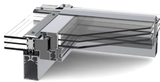
LAMILUX Ventilation Flap PR60 Variant 2
